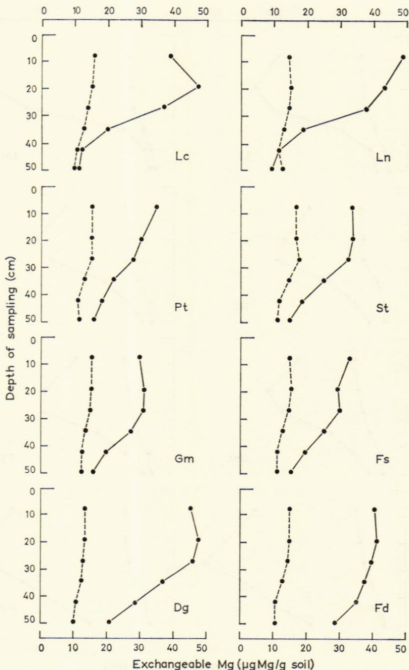
FIG. 2. Distribution of exchangeable Mg in soils sampled to 53 cm in 1964 (●---●---●) and in 1972/3 (●—●—●).
