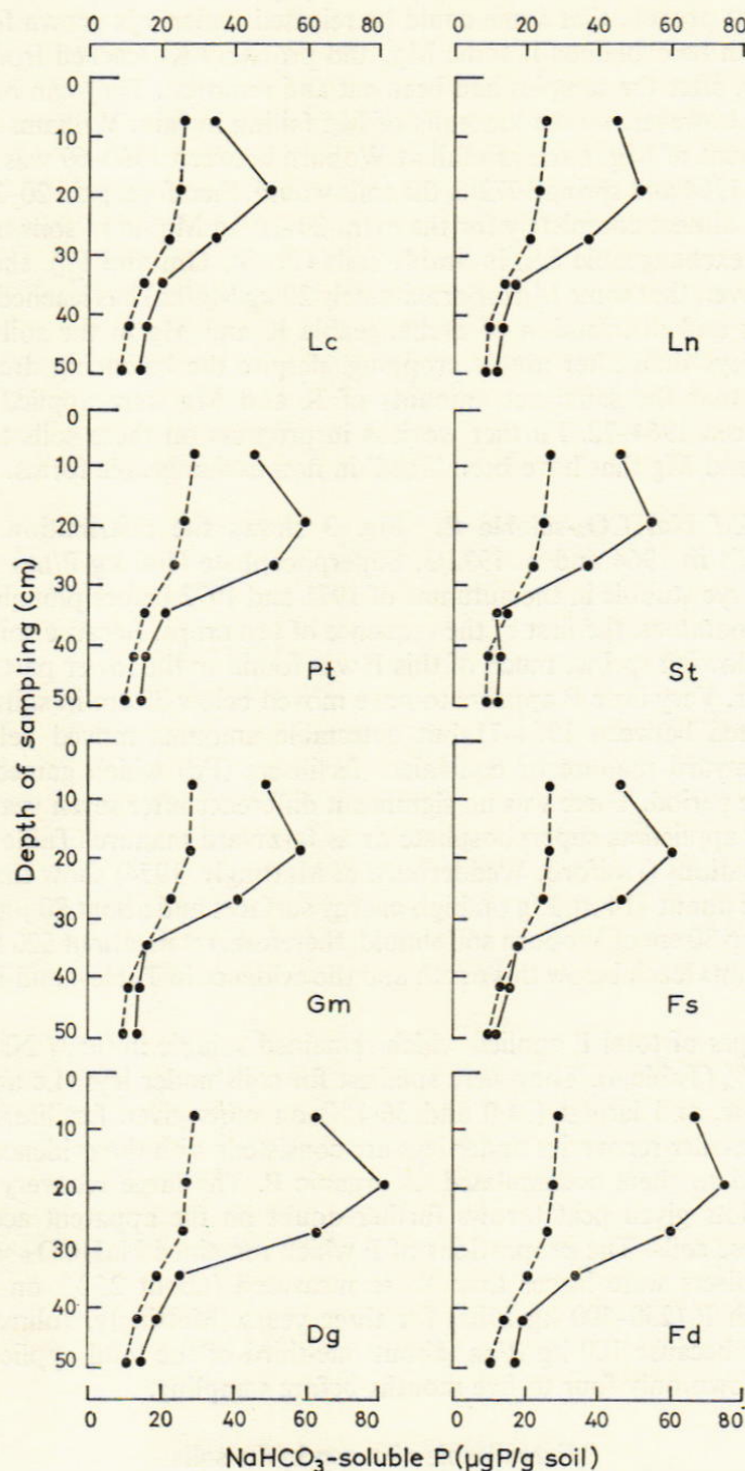
FIG. 3. Distribution of 0.5M sodium bicarbonate-soluble P in soils sampled to 53 cm in 1964 (●---●---●) and in 1972/3 (●—●—●).
