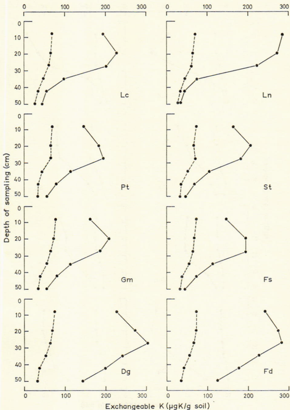
Fig. 1. Distribution of exchangeable K in soils sampled to 53 cm in 1964 (●---●---●) and in 1972/3 (●—●—●).
