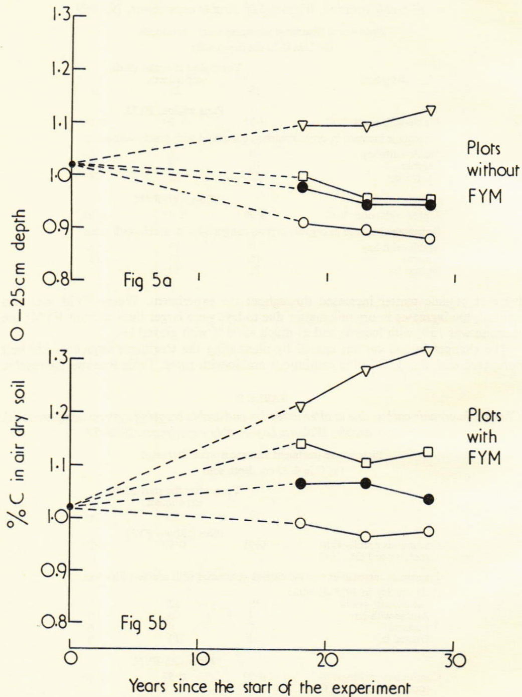
FIG. 5. Changes in organic carbon in soil caused by ley and arable cropping systems. Woburn Ley-Arable experiment, 1938-69. Plots where treatment sequences were continuous. FIG. 5a. Plots not given farmyard manure (FYM). FIG. 5b. Plots given farmyard manure, 38 t/ha once every five years. Cropping systems tested: arable-with-roots, ○; arable-with-hay, ●; lucerne, □; grazed ley, ▽.
