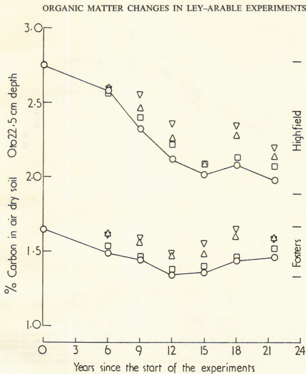
FIG. 1. Changes in organic carbon in soil caused by ley and arable cropping systems. Rothamsted Ley-Arable experiments, 1949-72. Continuous arable cropping, \circ ; ley-arable cropping systems, lucerne, \square ; cut grass/ley-with-N, \triangle ; grazed ley/ley-with-clover, \nabla . (Results are means from eight blocks for each experiment for 6, 9, 12 and 21/22 years and from four blocks for 15 and 18 years.)
