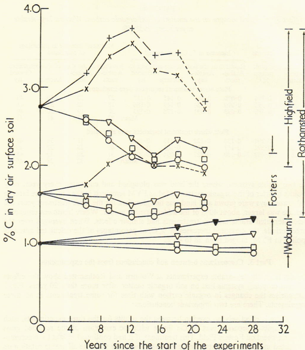
FIG. 7. Changes in organic carbon in soil caused by some of the cropping systems tested in three ley-arable experiments. (i) Woburn, where treatment sequences were continuous, 1938-69; (ii) Fosters field, Rothamsted, 1949-72; (iii) Highfield, Rothamsted, 1949-72. Continuous arable cropping, ○; ley-arable systems, lucerne, □; grazed ley, ▽; grazed ley with farmyard manure, ▼; grass for many years; reseeded grass, ×; permanent grass, +; these two grass treatments were divided into grass grazed, —; grass cut, — —; arable cropping after grass ploughed, - - - - -.
