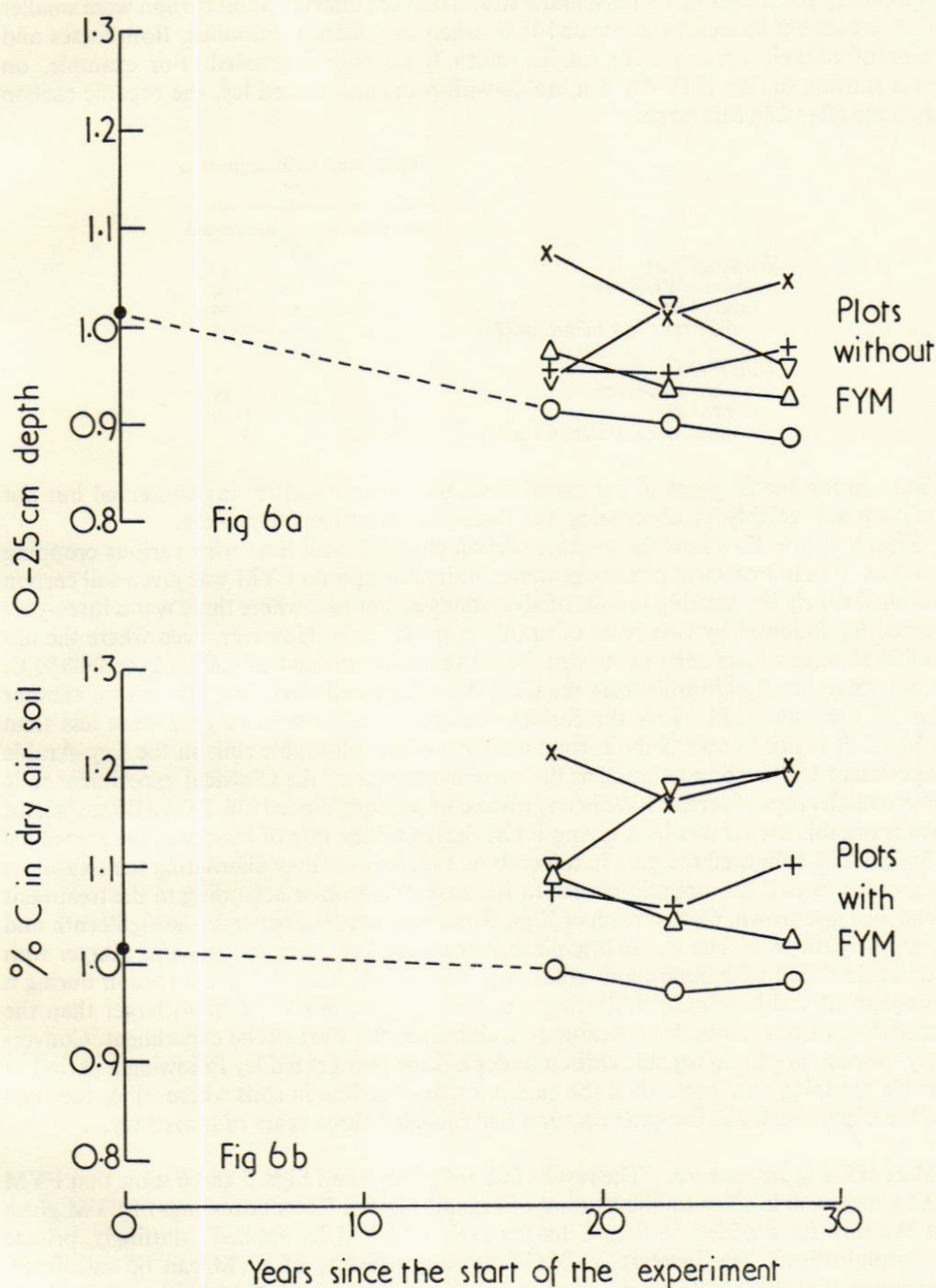
FIG. 6. Changes in organic carbon in soil caused by alternating the treatment sequences compared to the continuous arable-with-roots system. Woburn Ley-Arable experiment, 1938-69.
